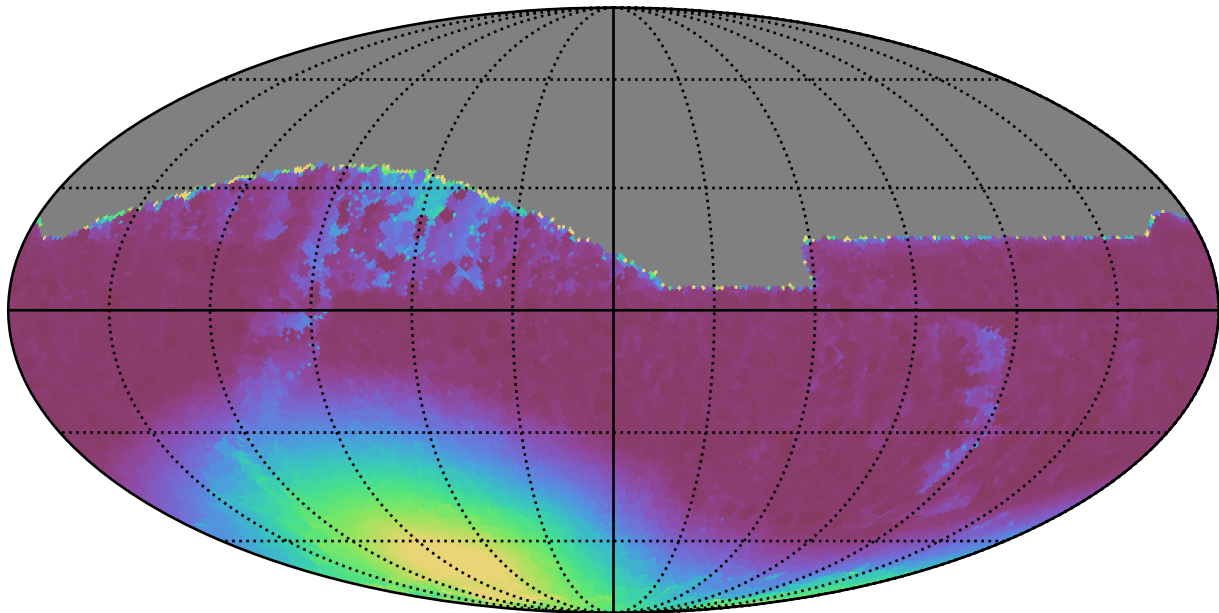
reweight_plane_v3.3_10yrs All sky z band: Min moonDistance
