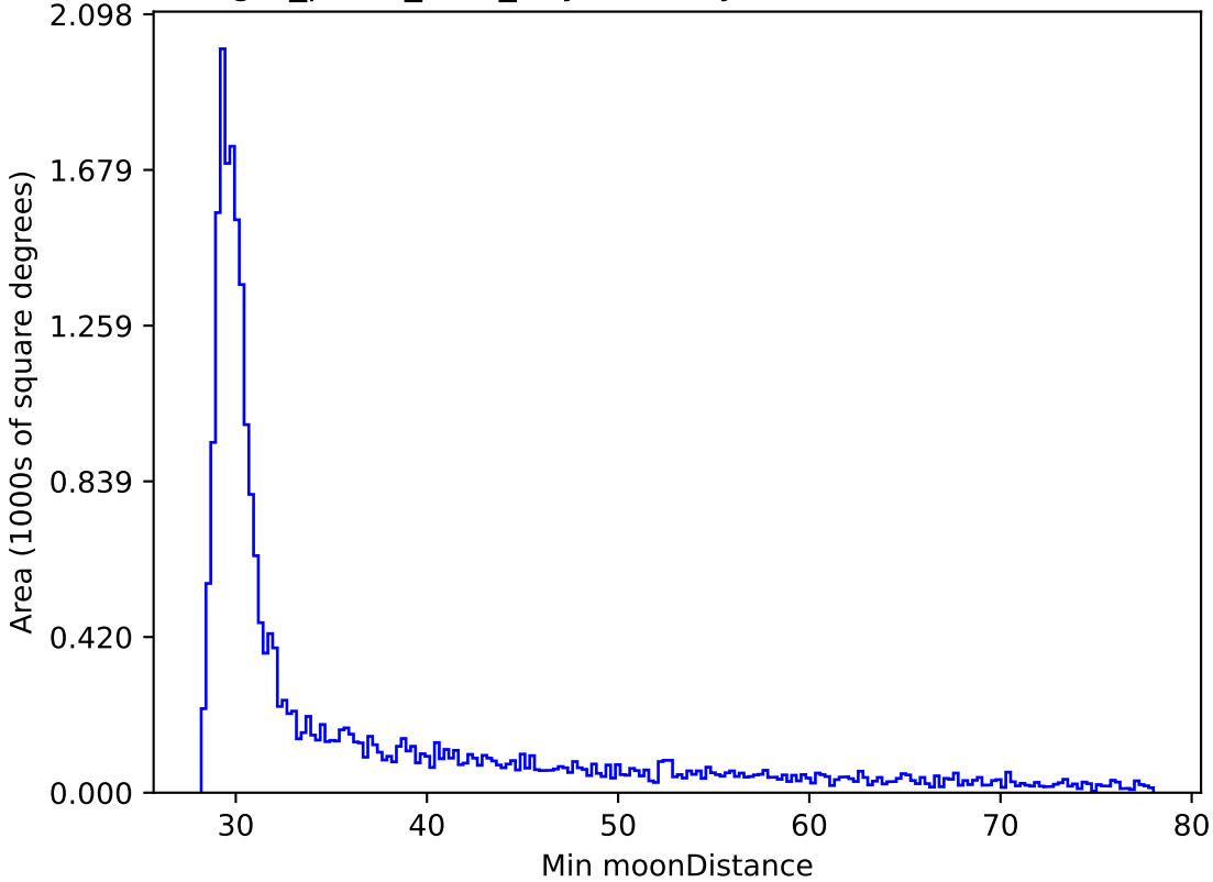
reweight_plane_v3.3_10yrs All sky z band: Min moonDistance
