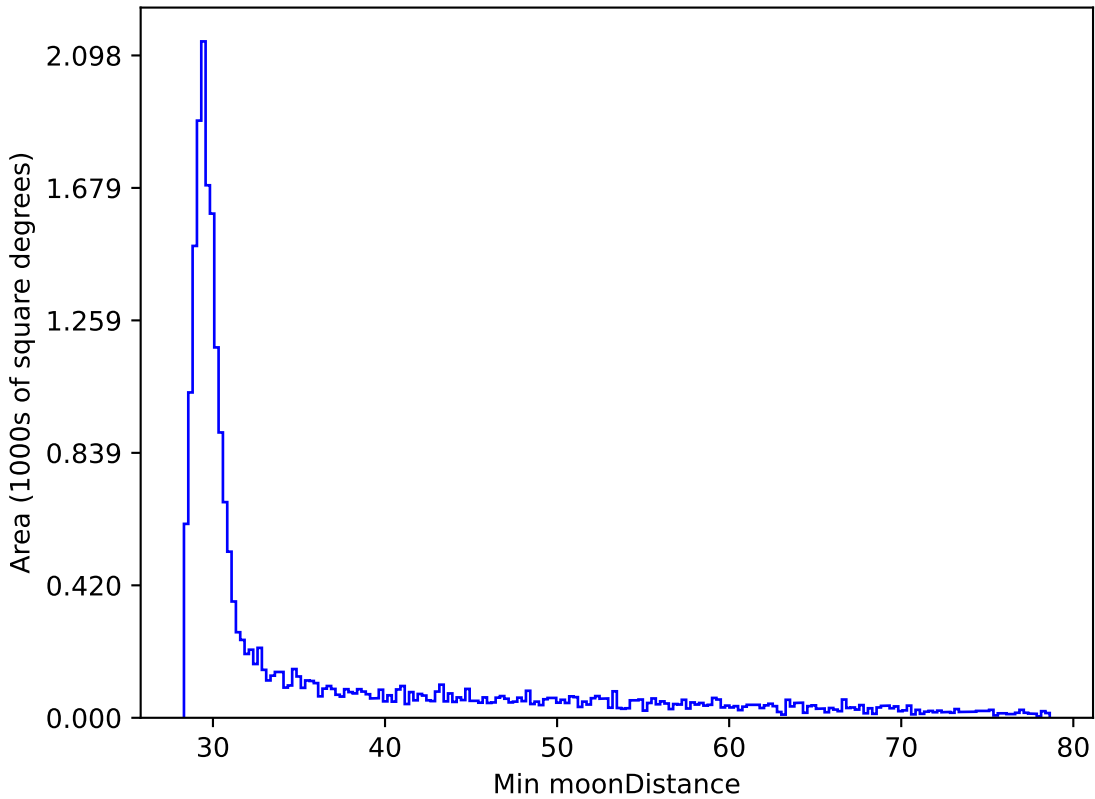
reweight_plane_v3.3_10yrs All sky y band: Min moonDistance
