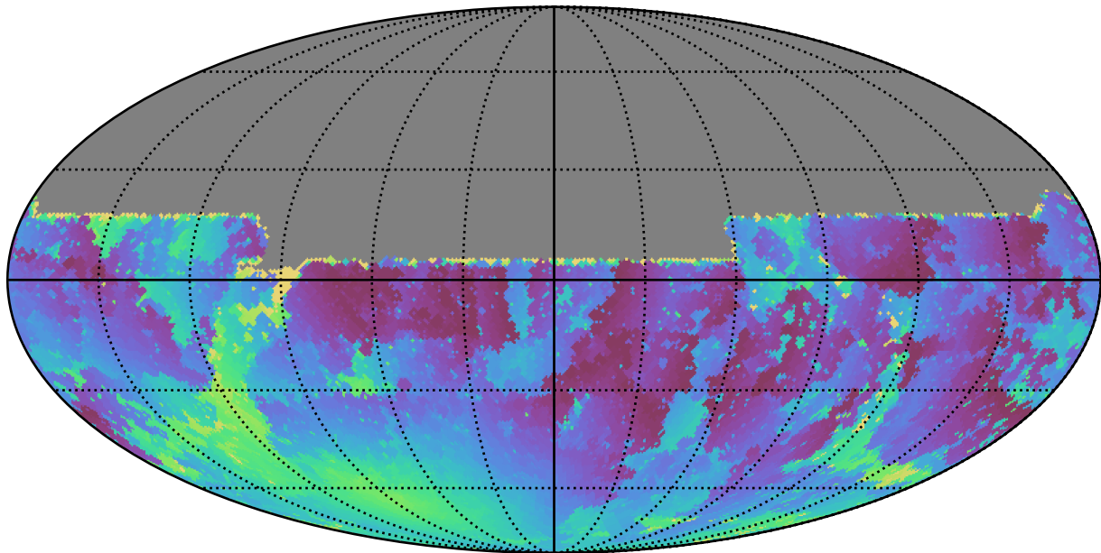
reweight_plane_v3.3_10yrs All sky u band: Min moonDistance
