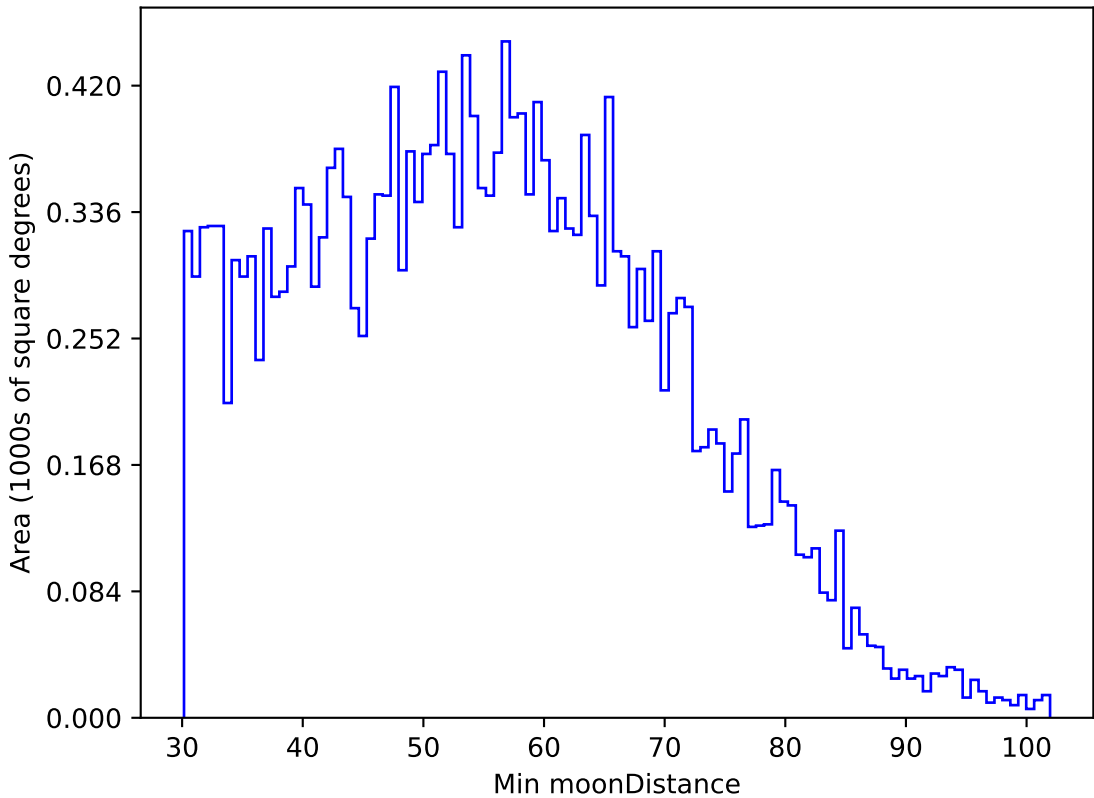
reweight_plane_v3.3_10yrs All sky u band: Min moonDistance
