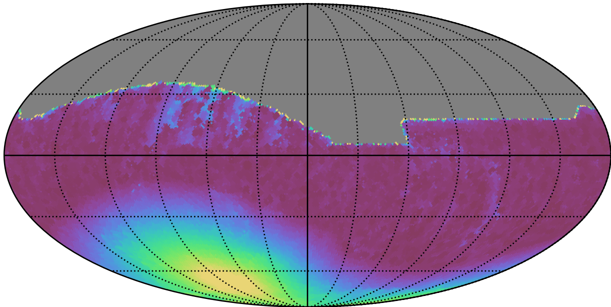
reweight_plane_v3.3_10yrs All sky i band: Min moonDistance
