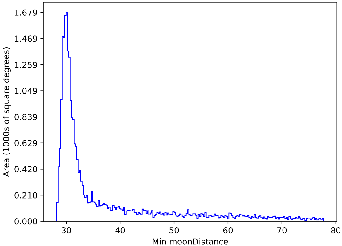
reweight_plane_v3.3_10yrs All sky i band: Min moonDistance
