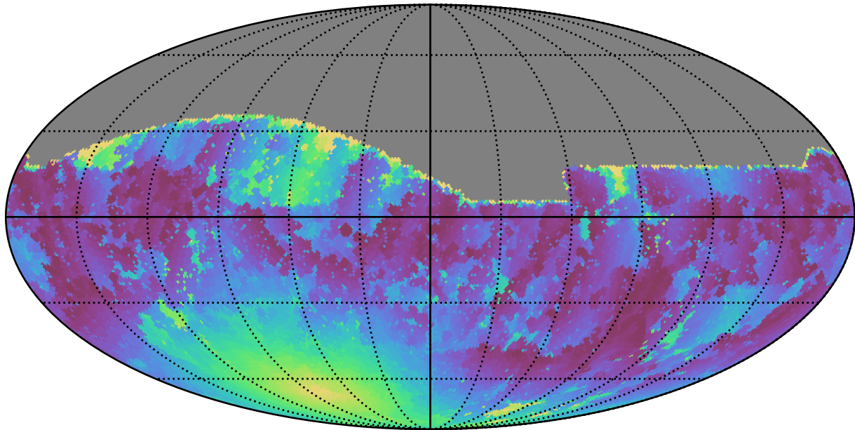
reweight_plane_v3.3_10yrs All sky g band: Min moonDistance
