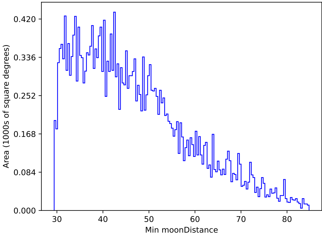
reweight_plane_v3.3_10yrs All sky g band: Min moonDistance
