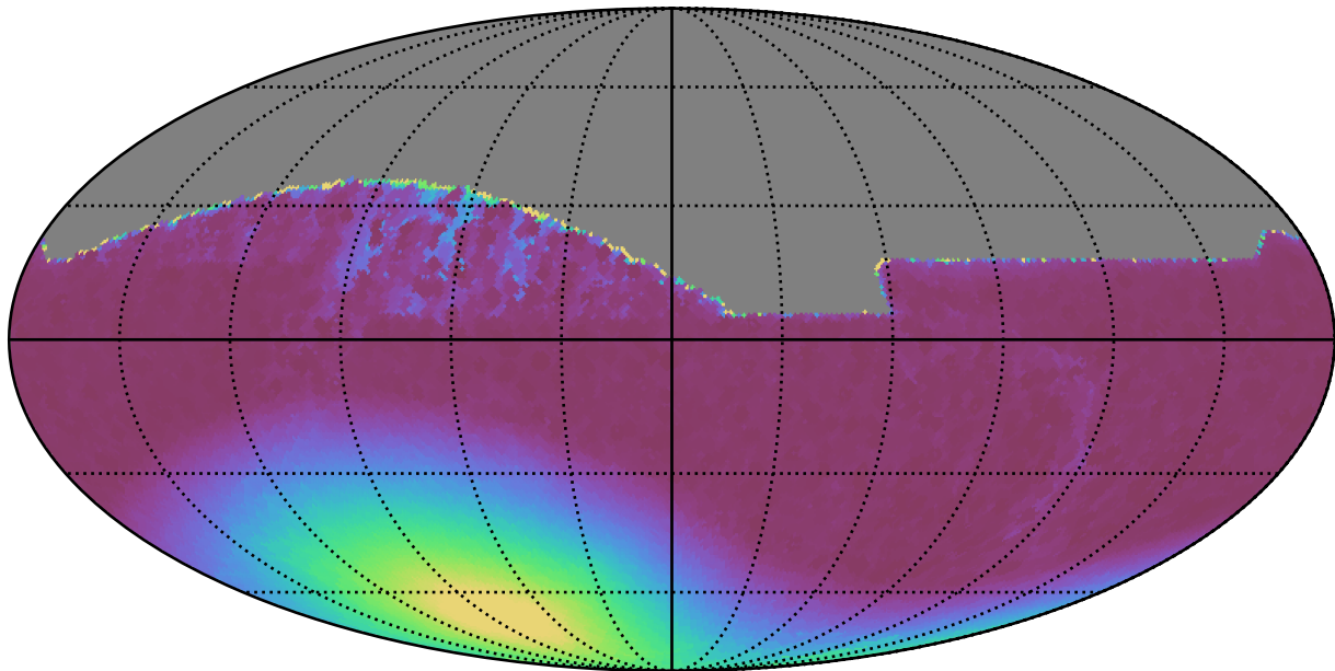
reweight_plane_v3.3_10yrs All sky all bands: Min moonDistance
