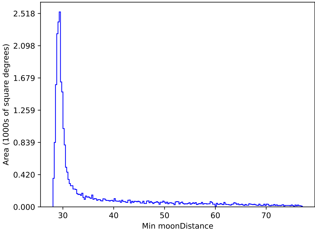
reweight_plane_v3.3_10yrs All sky all bands: Min moonDistance
