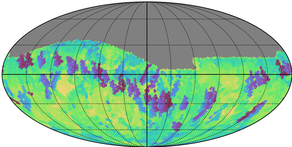
reweight_plane_v3.3_10yrs Yr 1 z band: Min fiveSigmaDepth
