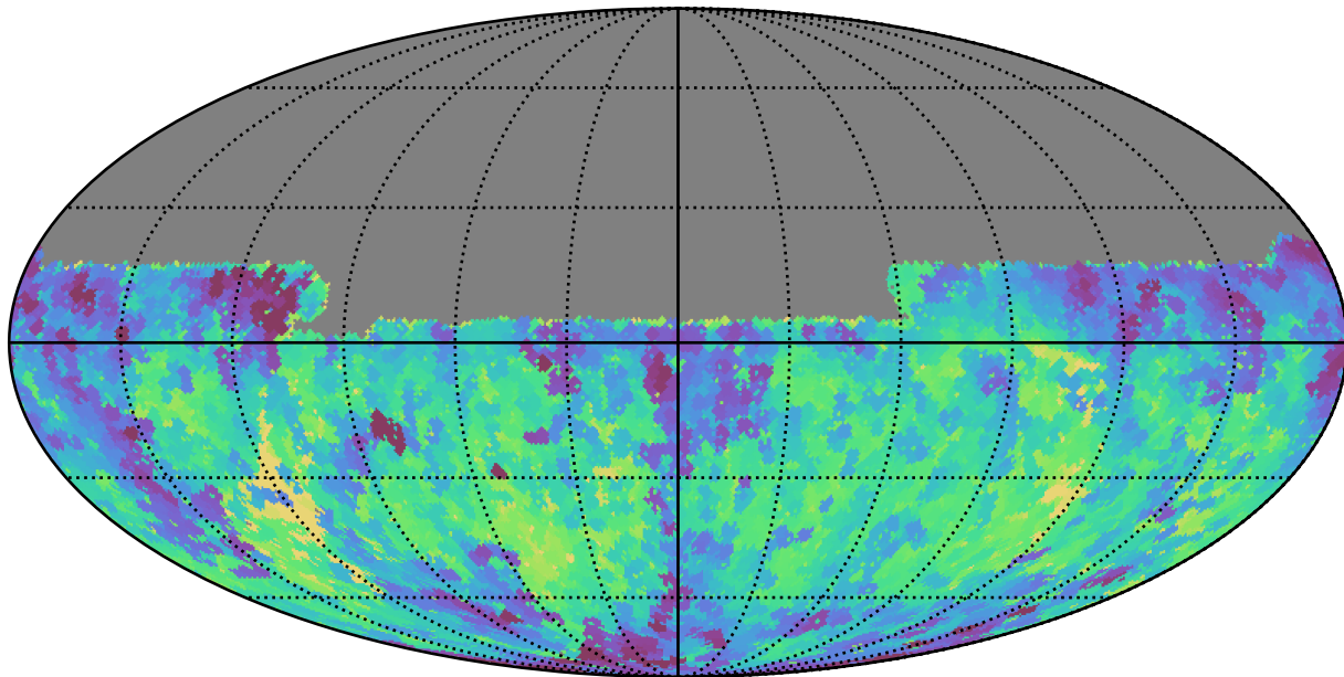
reweight_plane_v3.3_10yrs Yr 1 y band: Min fiveSigmaDepth
