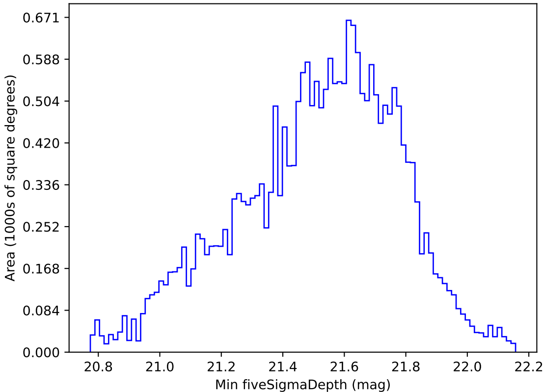
reweight_plane_v3.3_10yrs Yr 1 y band: Min fiveSigmaDepth
