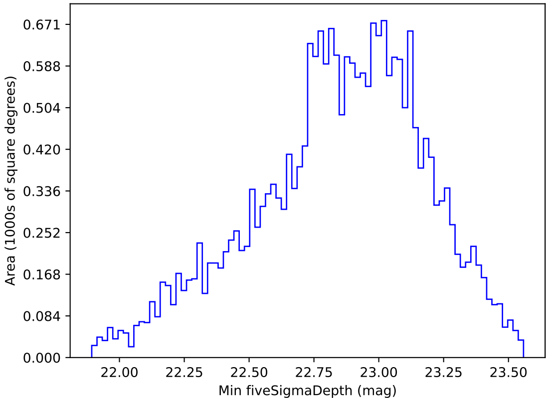
reweight_plane_v3.3_10yrs Yr 1 u band: Min fiveSigmaDepth
