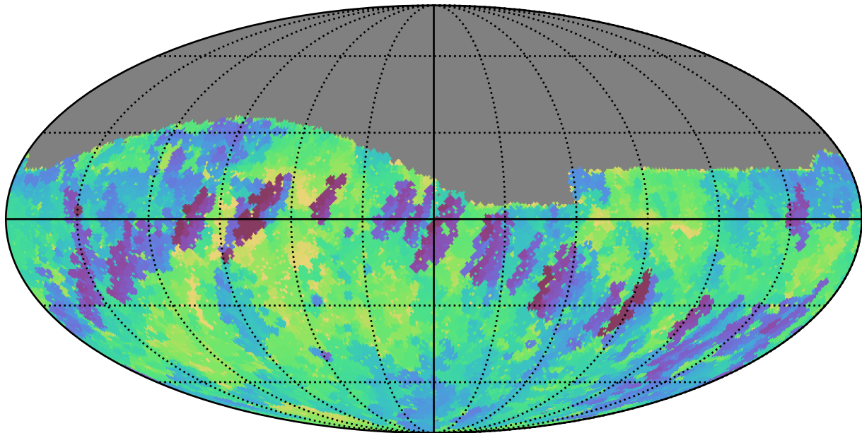
reweight_plane_v3.3_10yrs Yr 1 r band: Min fiveSigmaDepth
