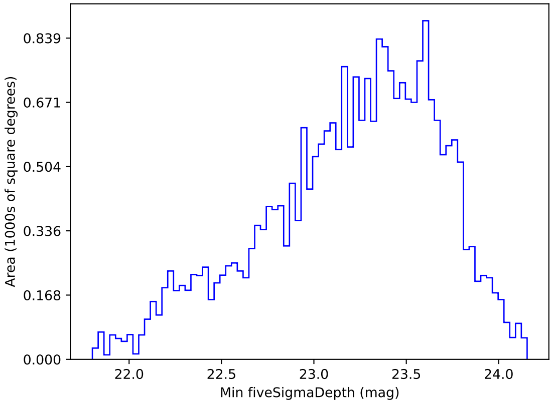
reweight_plane_v3.3_10yrs Yr 1 r band: Min fiveSigmaDepth
