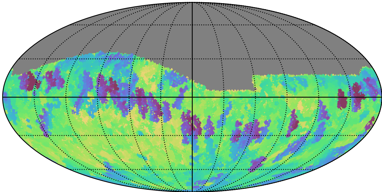
reweight_plane_v3.3_10yrs Yr 1 i band: Min fiveSigmaDepth
