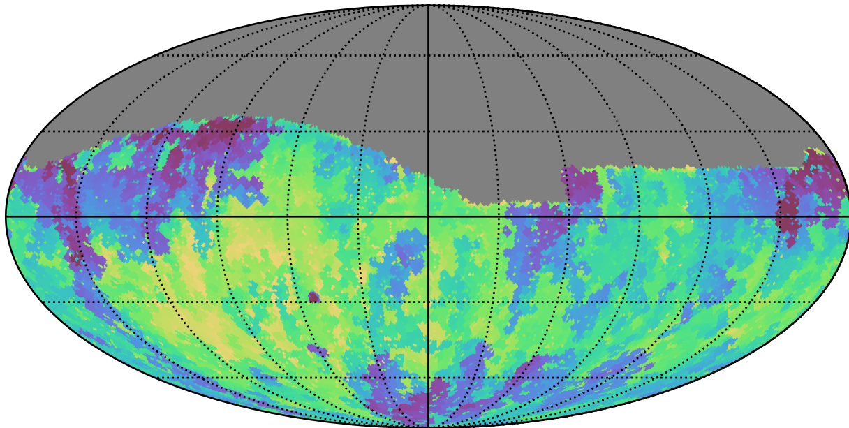
reweight_plane_v3.3_10yrs Yr 1 g band: Min fiveSigmaDepth
