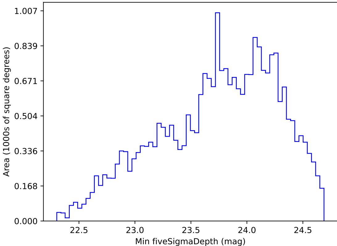
reweight_plane_v3.3_10yrs Yr 1 g band: Min fiveSigmaDepth
