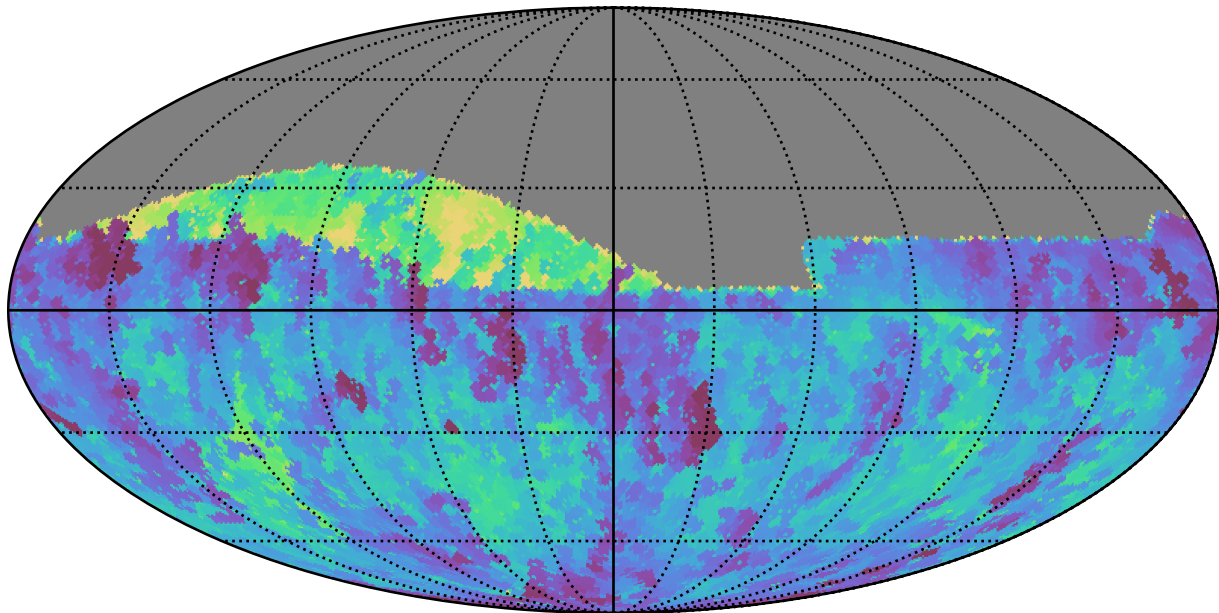
reweight_plane_v3.3_10yrs Yr 1 all bands: Min fiveSigmaDepth
