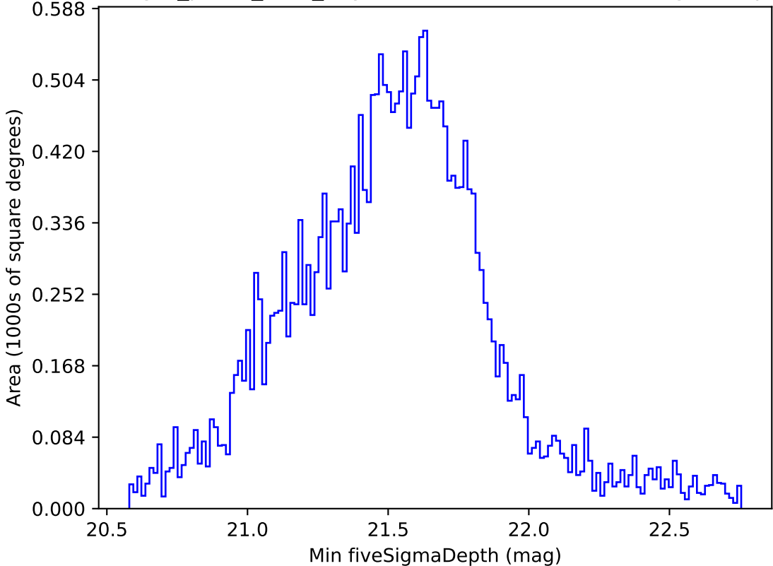
reweight_plane_v3.3_10yrs Yr 1 all bands: Min fiveSigmaDepth
