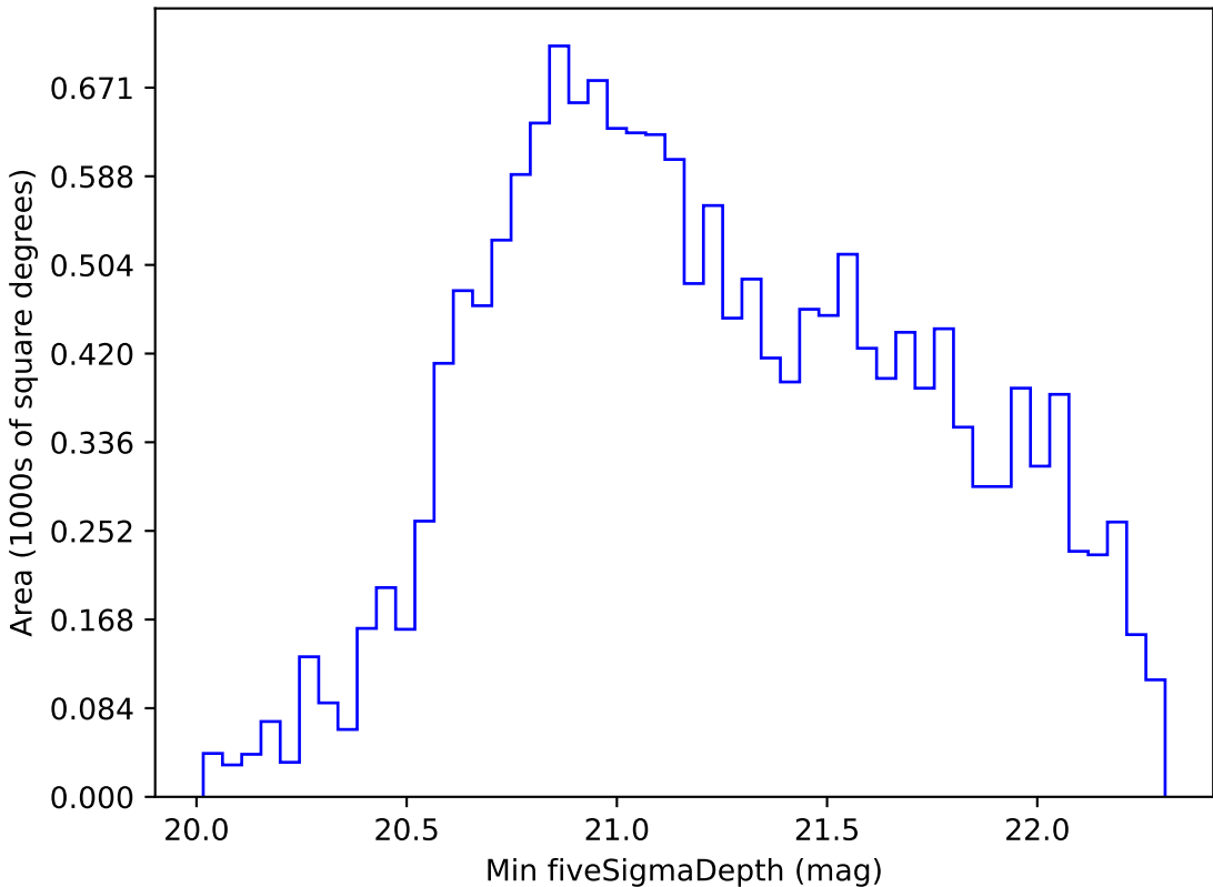
reweight_plane_v3.3_10yrs WFD z band: Min fiveSigmaDepth
