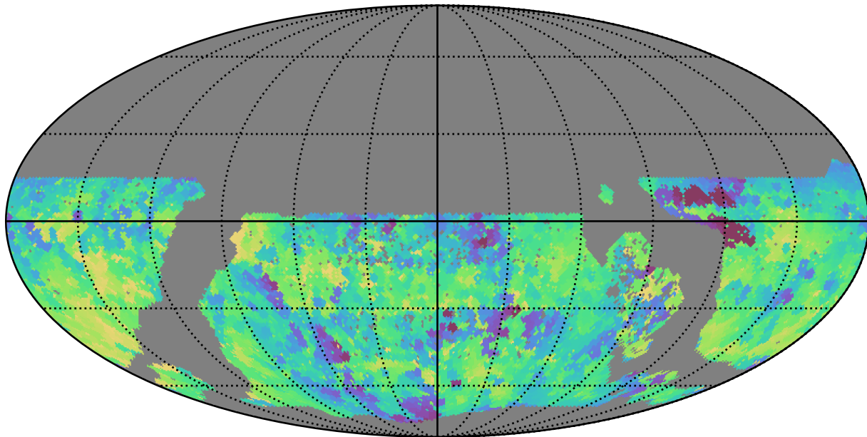
reweight_plane_v3.3_10yrs WFD u band: Min fiveSigmaDepth
