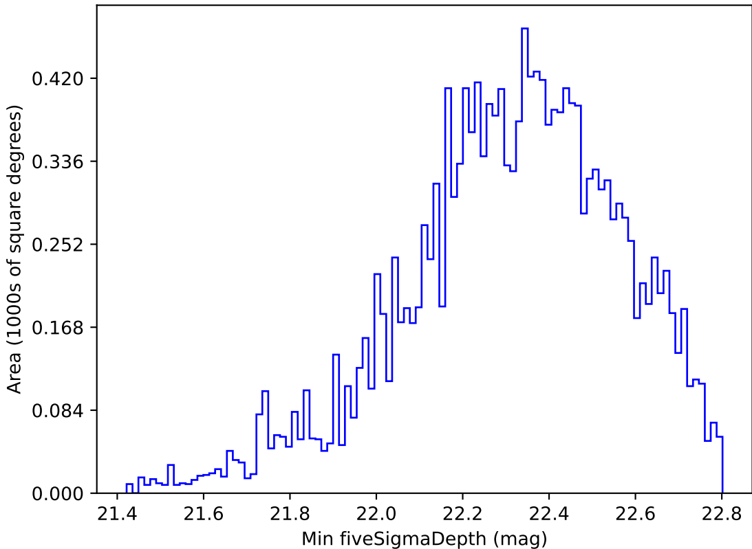
reweight_plane_v3.3_10yrs WFD u band: Min fiveSigmaDepth
