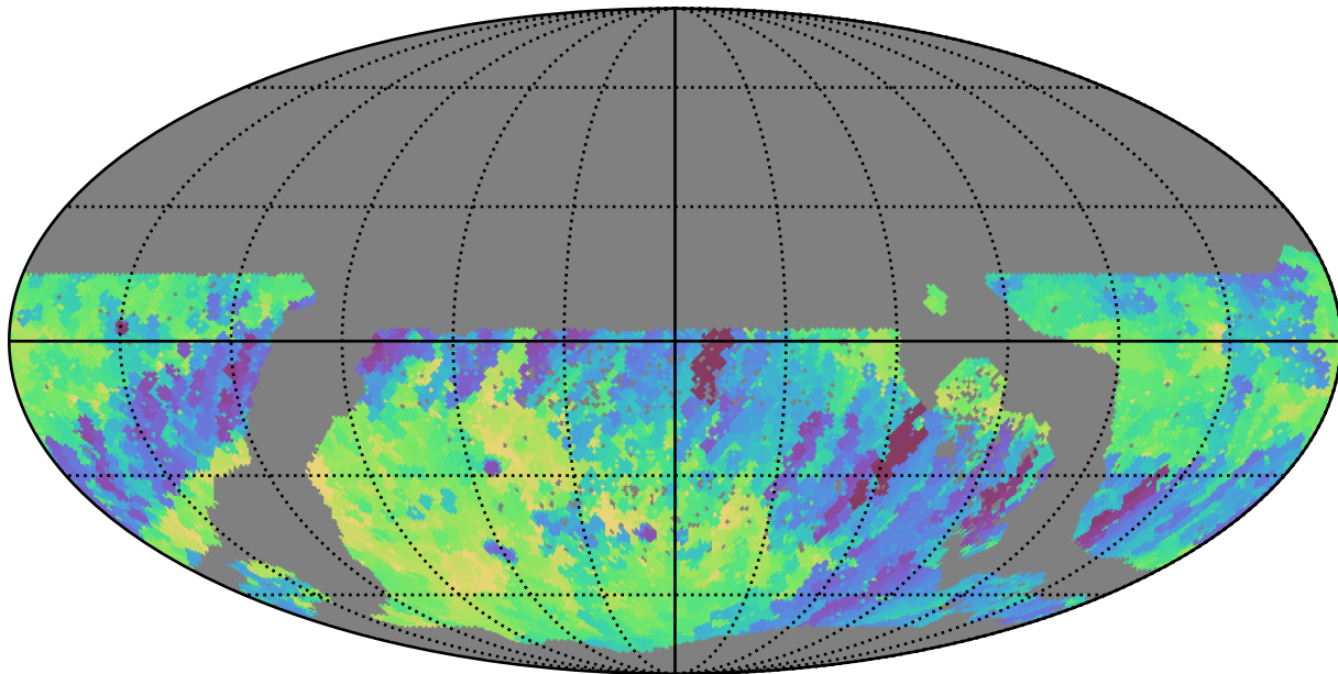
reweight_plane_v3.3_10yrs WFD r band: Min fiveSigmaDepth
