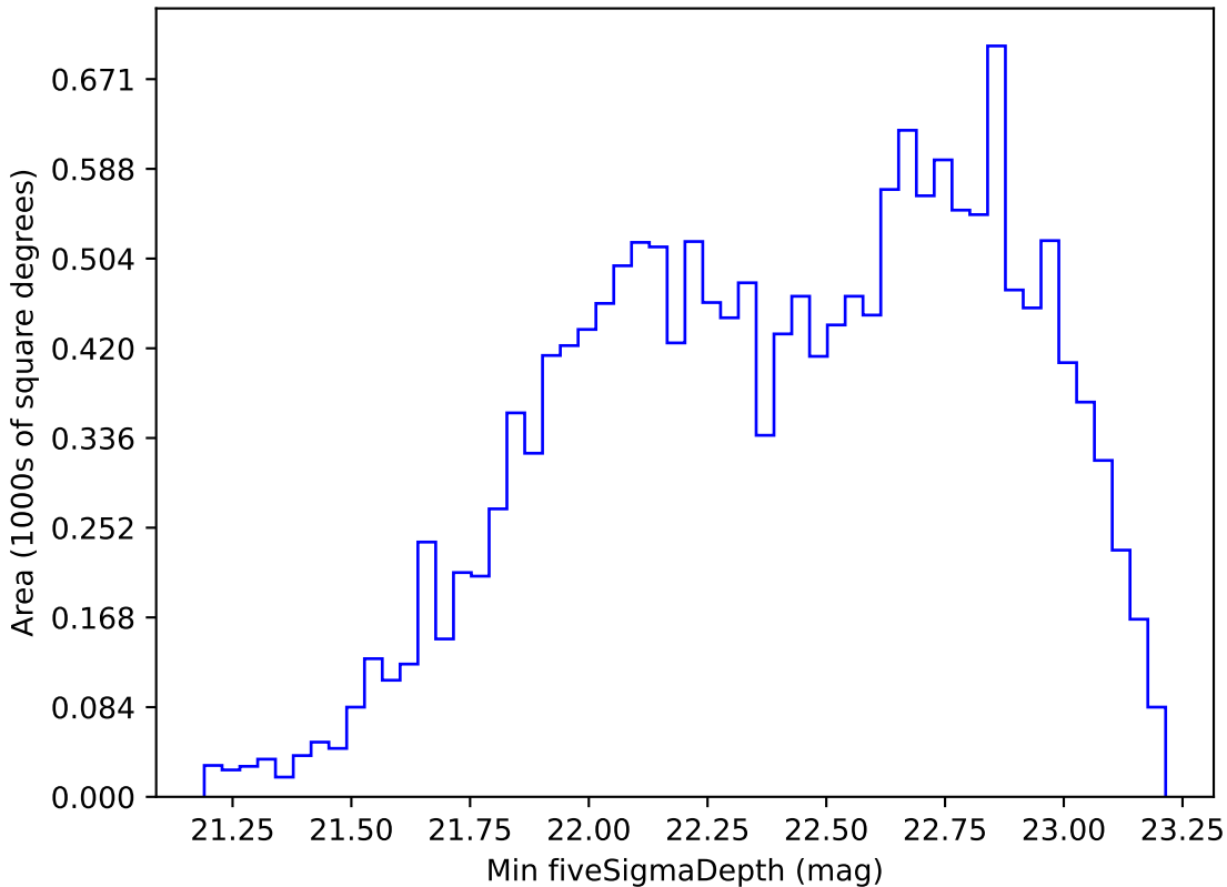
reweight_plane_v3.3_10yrs WFD r band: Min fiveSigmaDepth
