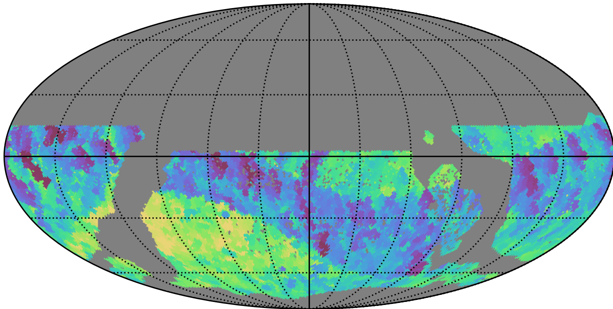
reweight_plane_v3.3_10yrs WFD i band: Min fiveSigmaDepth
