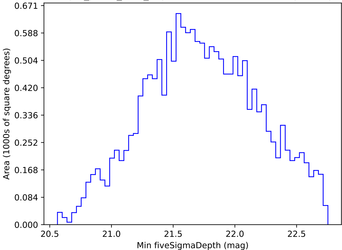
reweight_plane_v3.3_10yrs WFD i band: Min fiveSigmaDepth
