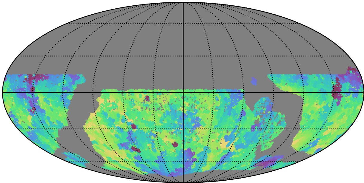
reweight_plane_v3.3_10yrs WFD g band: Min fiveSigmaDepth
