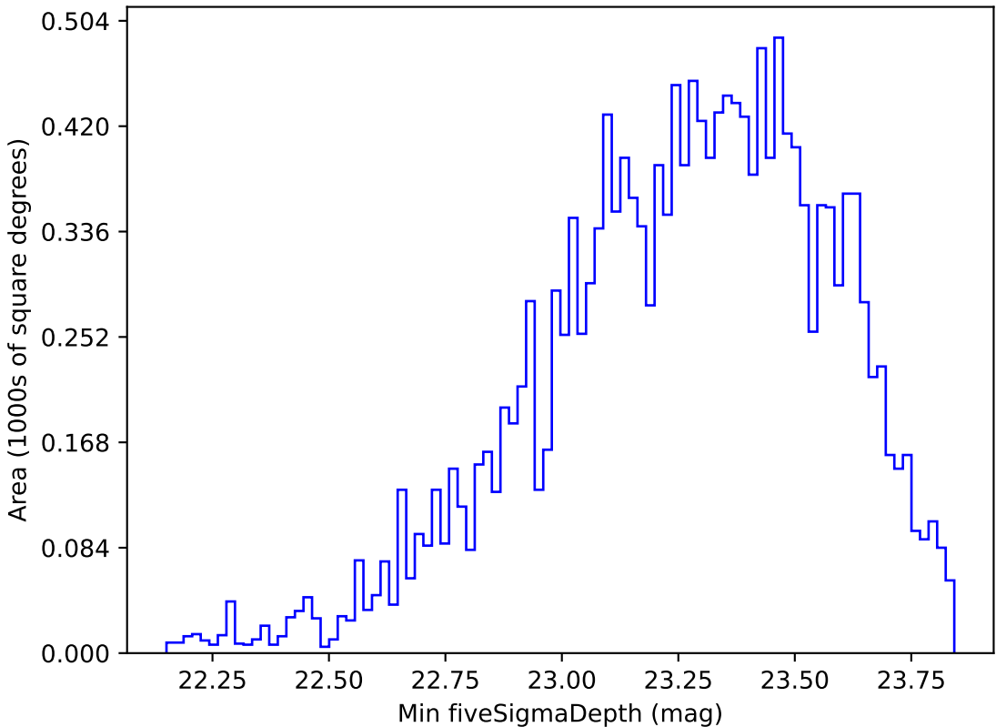
reweight_plane_v3.3_10yrs WFD g band: Min fiveSigmaDepth
