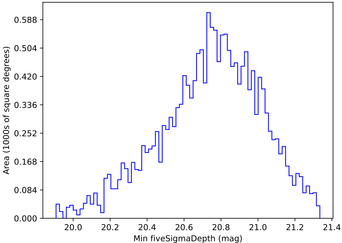
reweight_plane_v3.3_10yrs WFD all bands: Min fiveSigmaDepth
