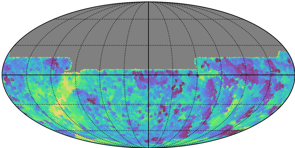
reweight_plane_v3.3_10yrs All sky y band: Min fiveSigmaDepth
