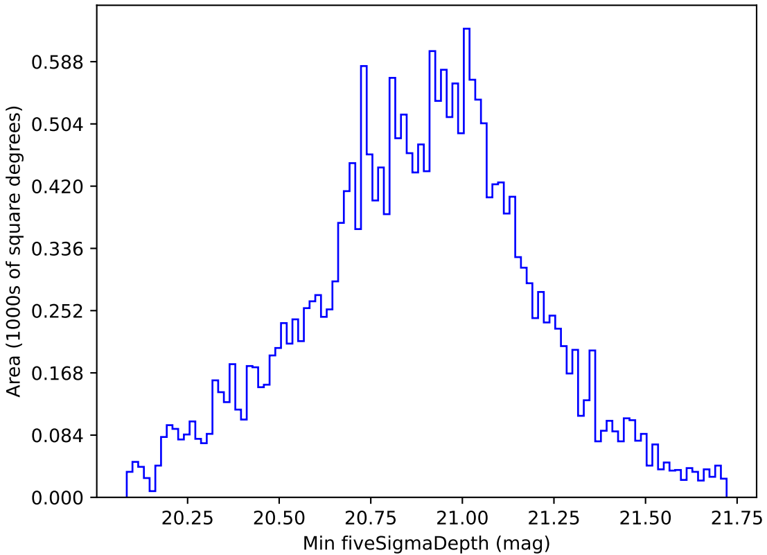
reweight_plane_v3.3_10yrs All sky y band: Min fiveSigmaDepth
