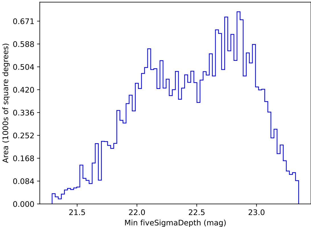
reweight_plane_v3.3_10yrs All sky r band: Min fiveSigmaDepth
