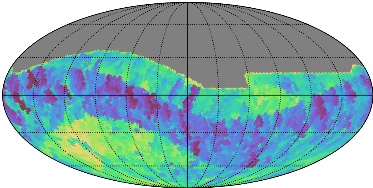
reweight_plane_v3.3_10yrs All sky i band: Min fiveSigmaDepth
