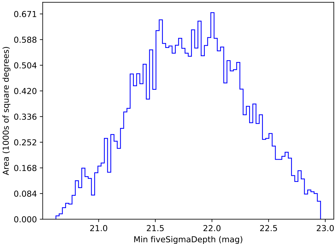
reweight_plane_v3.3_10yrs All sky i band: Min fiveSigmaDepth
