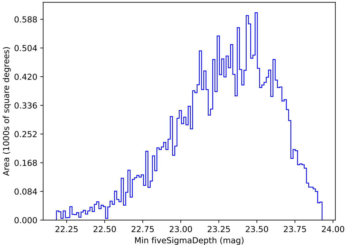
reweight_plane_v3.3_10yrs All sky g band: Min fiveSigmaDepth
