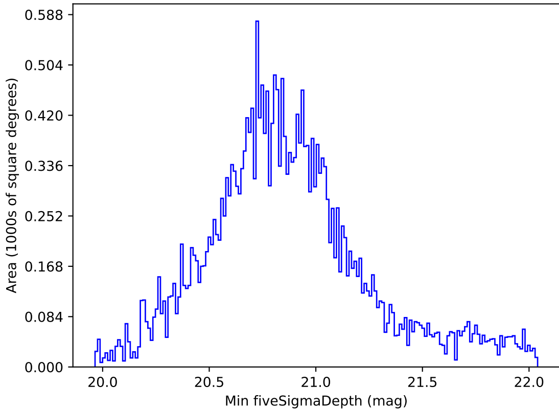
reweight_plane_v3.3_10yrs All sky all bands: Min fiveSigmaDepth
