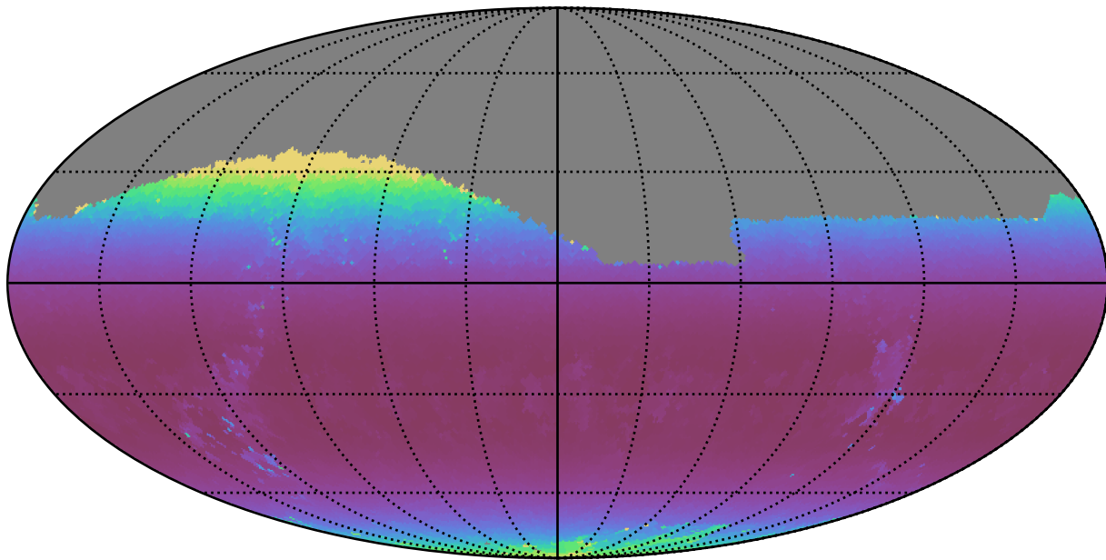
reweight_plane_v3.3_10yrs Yr 1 z band: Min airmass
