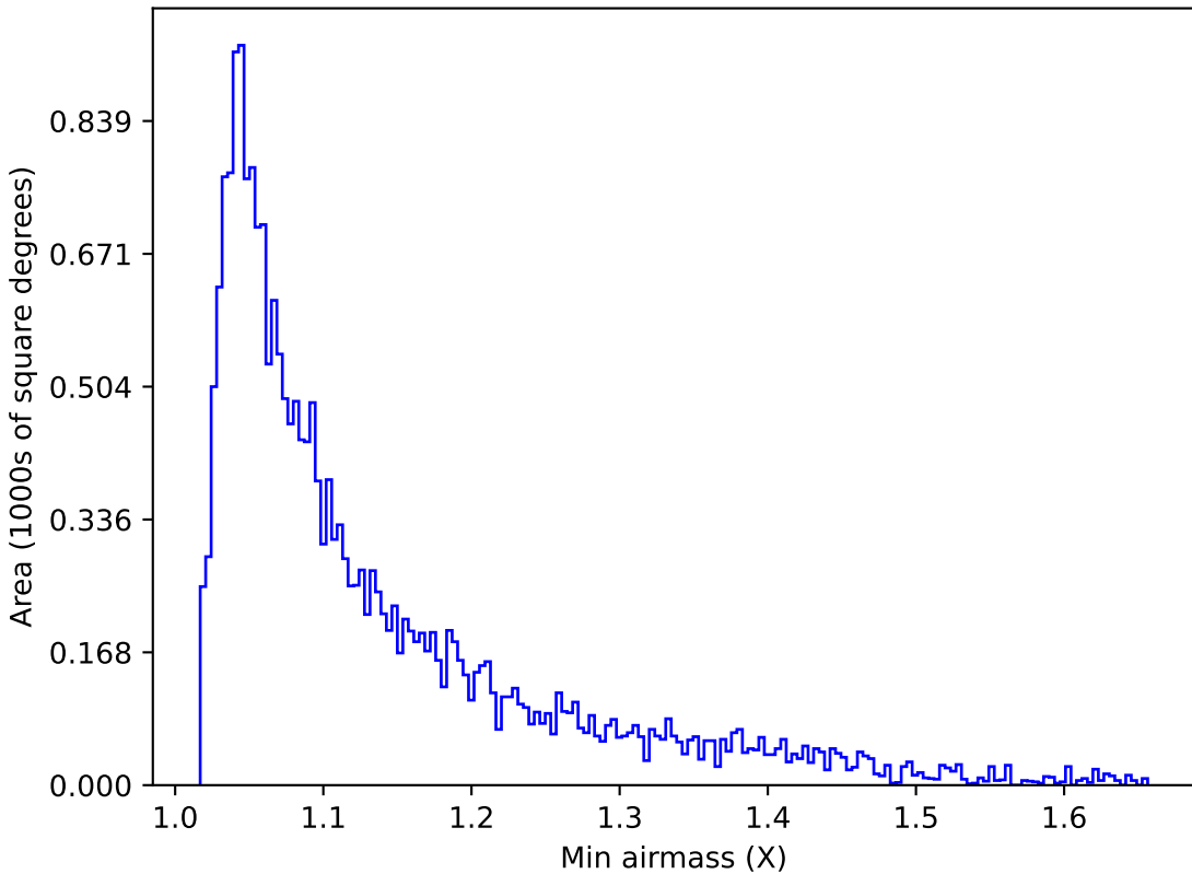
reweight_plane_v3.3_10yrs Yr 1 u band: Min airmass
