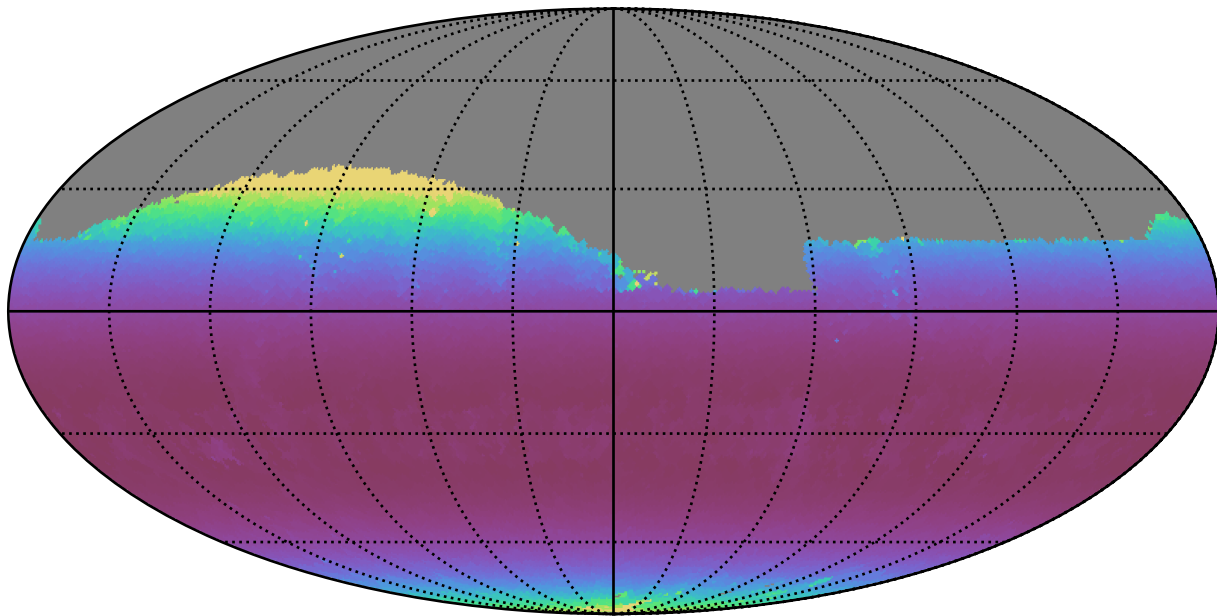
reweight_plane_v3.3_10yrs Yr 1 r band: Min airmass
