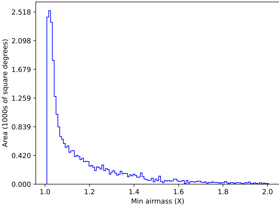
reweight_plane_v3.3_10yrs Yr 1 i band: Min airmass
