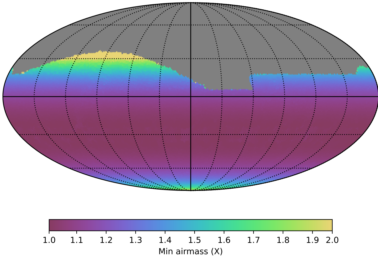
reweight_plane_v3.3_10yrs Yr 1 all bands: Min airmass
