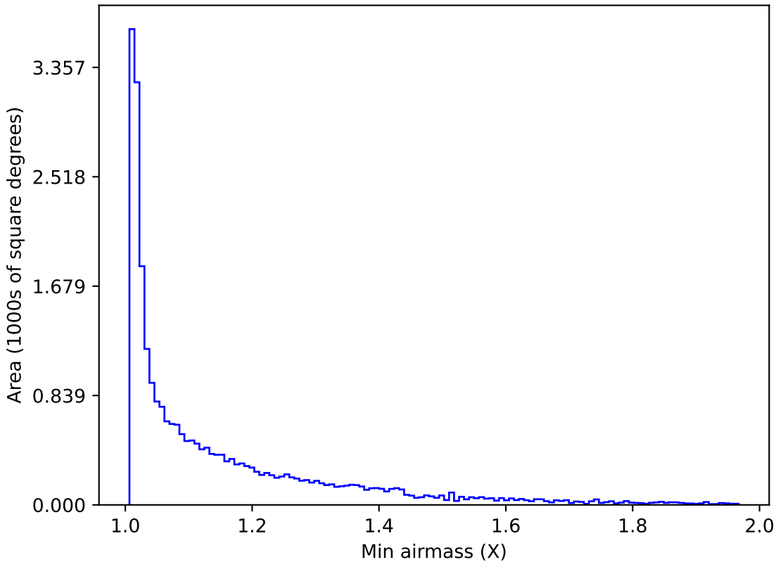
reweight_plane_v3.3_10yrs Yr 1 all bands: Min airmass
