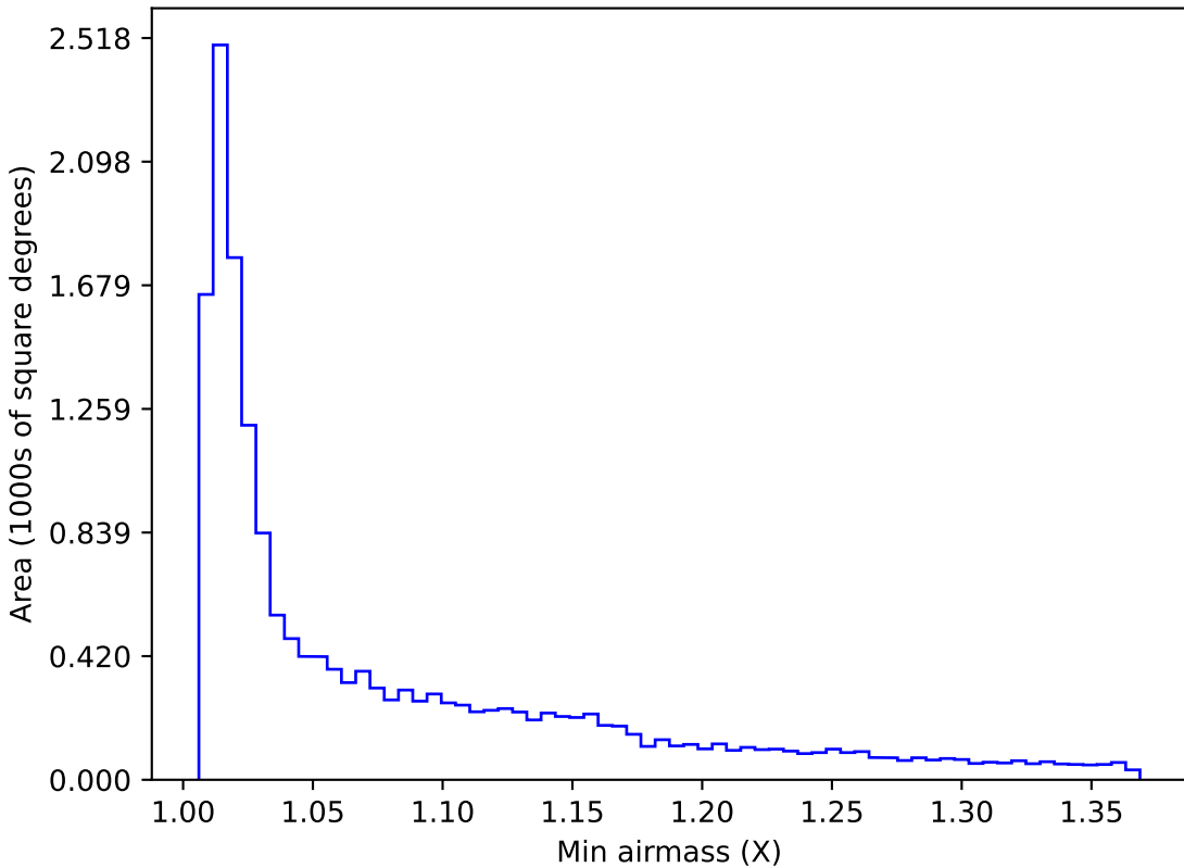
reweight_plane_v3.3_10yrs WFD y band: Min airmass
