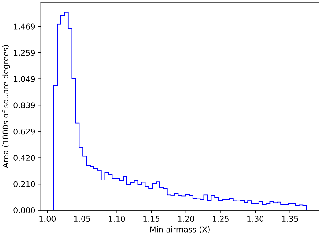
reweight_plane_v3.3_10yrs WFD u band: Min airmass
