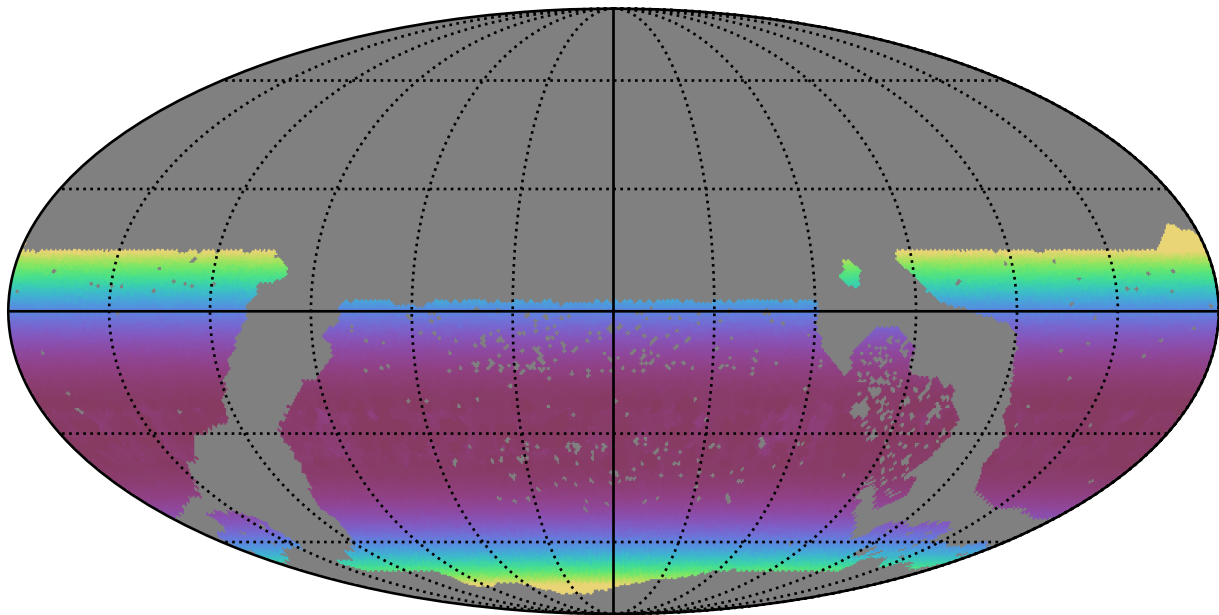
reweight_plane_v3.3_10yrs WFD r band: Min airmass
