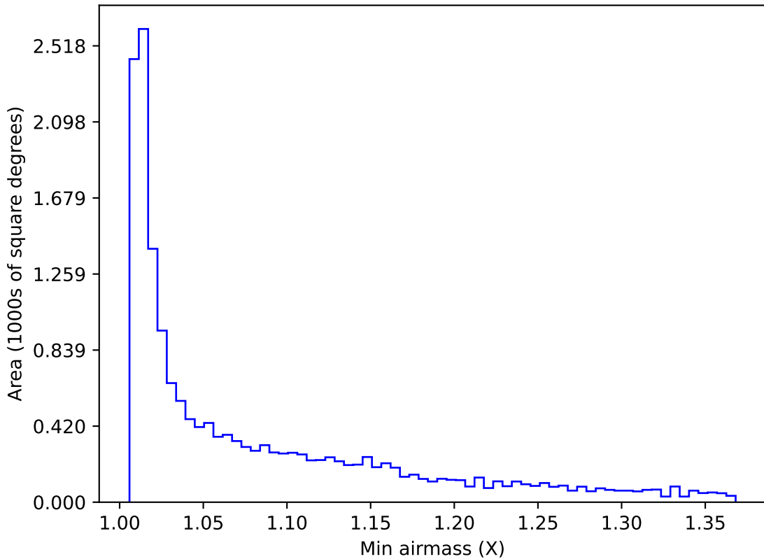
reweight_plane_v3.3_10yrs WFD r band: Min airmass
