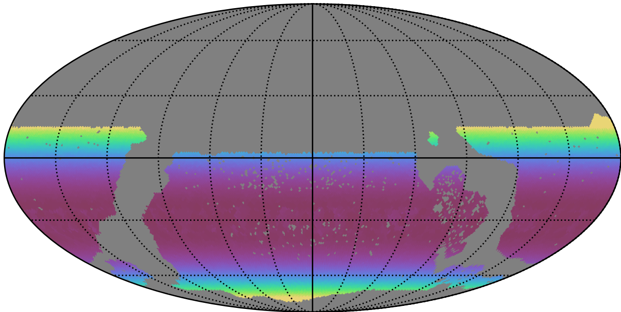
reweight_plane_v3.3_10yrs WFD i band: Min airmass
